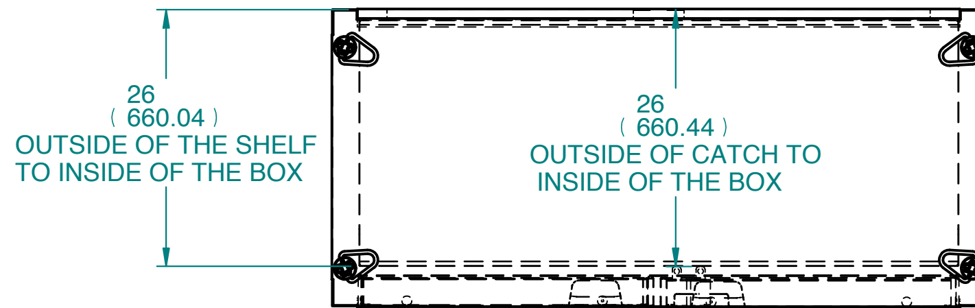
TOP VIEW
