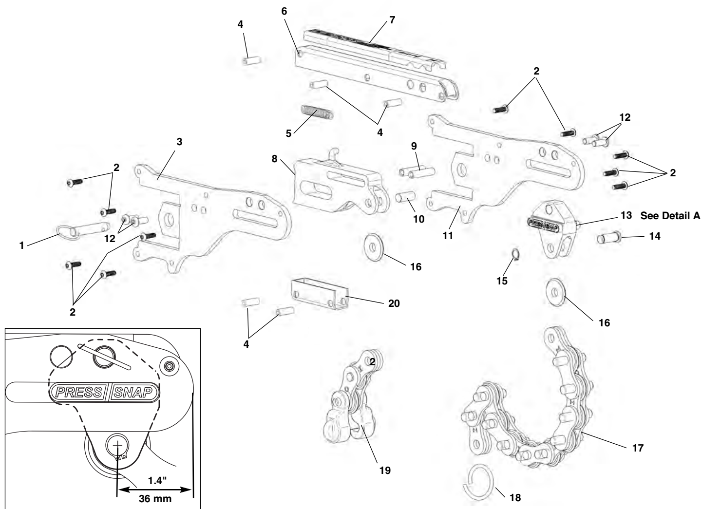
Detail A
